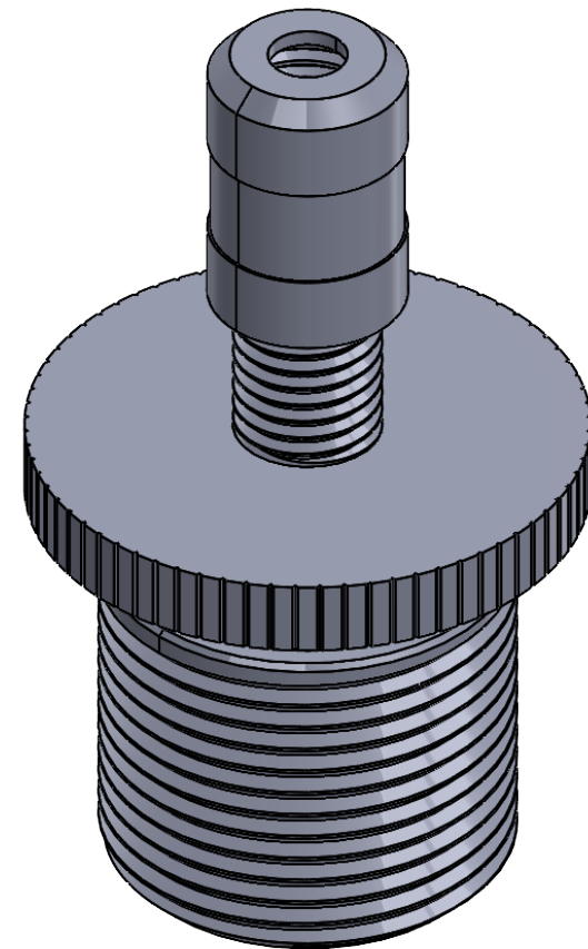
ISO VIEW SCALE 3 : 1
